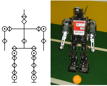
Fig. 1. Left: Kinematic structure of the robots. Right: Humanoid Robot Bruno (DD2008 model).
