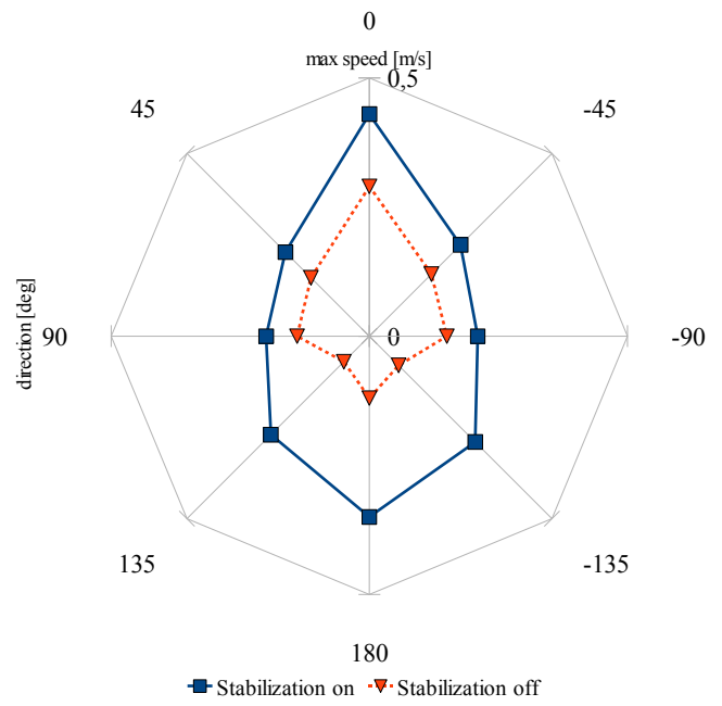
Fig. 11. Maximum Walking Speeds for DD2008
