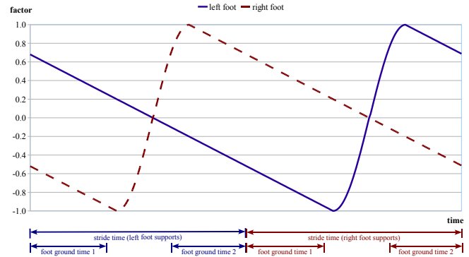
Fig. 5. X-Axis Motion Table: the factor to be multiplied with the stride length plottet over time for a double stride
