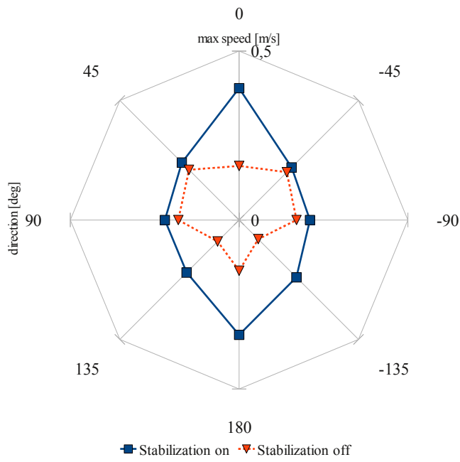
Fig. 10. Maximum Walking Speeds for DD2007
