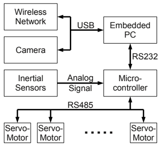
Fig. 2. Integration of the robot's computers, sensors and servo-motors.
