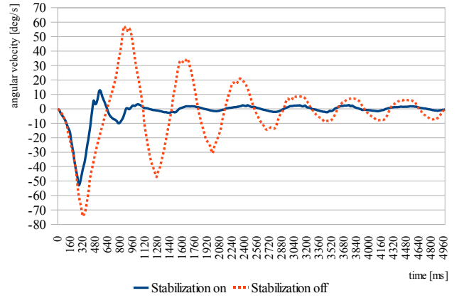
Fig. 8. Pitch Stabilization on a DD2008: angular velocity measured by the pitch axis gyroscope for 5 seconds
