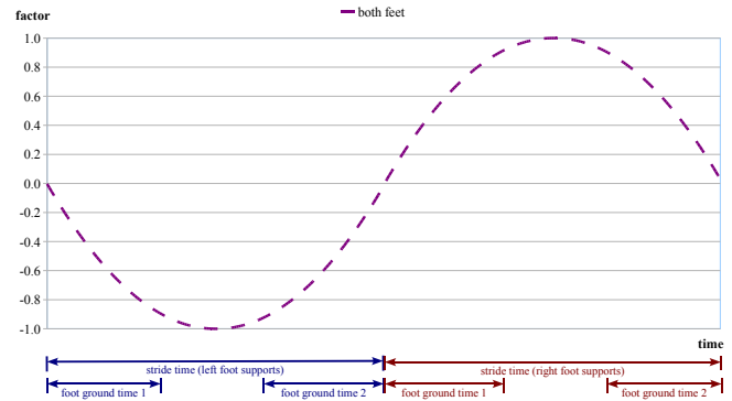
Fig. 6. Y-Axis Motion Table: the factor to be multiplied with the stride width plottet over time for a double stride
