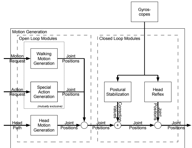
Fig. 3. Structure of the motion generation. At empty circles joint positions coming from above may override joint angles coming from the left.
