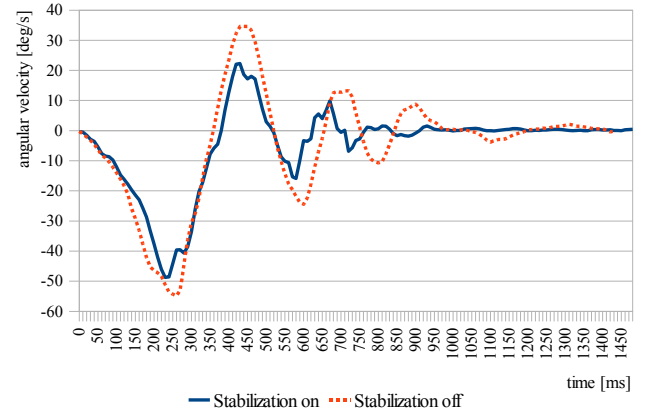
Fig. 9. Roll Stabilization on a DD2008: angular velocity measured by the roll axis gyroscope for 1.5 seconds
