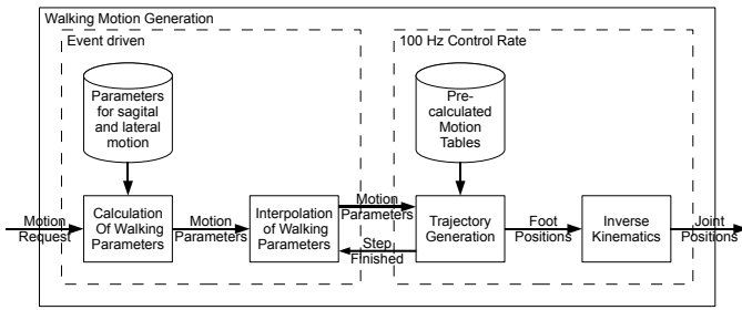
Fig. 4. Structure of the open loop walking motion generation.
