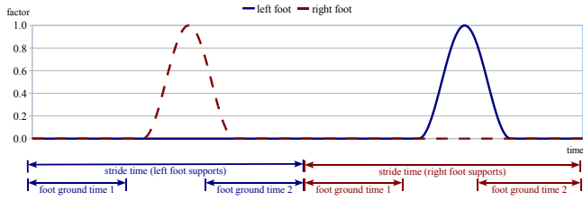
Fig. 7. Z-Axis Motion Table: the factor to be multiplied with the stride height plottet over time for a double stride
